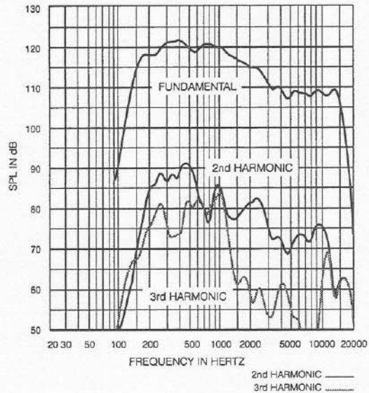
FIGURE 6 — MTH-2.5/22B Harmonic Distortion
